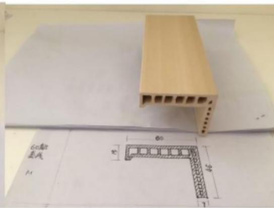
6046直边线条 6046 Straight Architrave.
