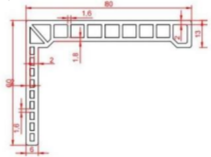
8060直边线条 8060 Straight Architrave
