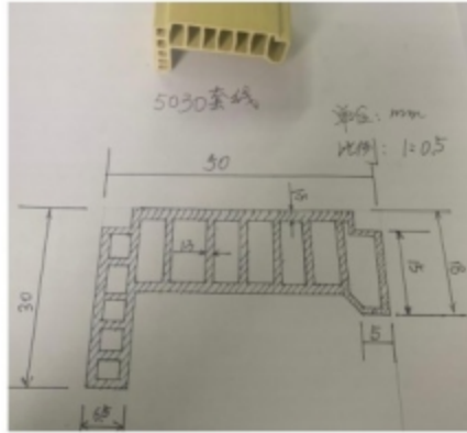
5030线条 5030 Architrave
