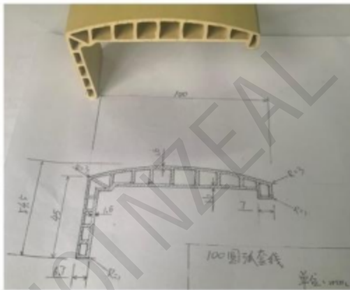
1054弧形线条 1054 Curved Architrave
