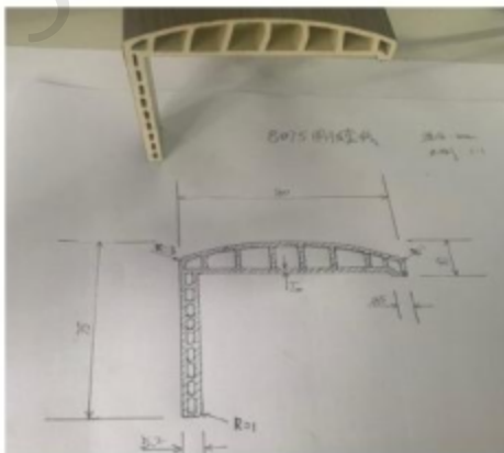
8075弧形线条 8075 Curved Architrave
